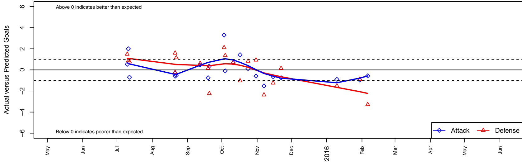
ISC Gunners Select B97 Dots are actual minus expected GF (blue circles) and GA (red triangles). Blue line is smoothed change in attack strength. Red is smoothed change in defense strength.
